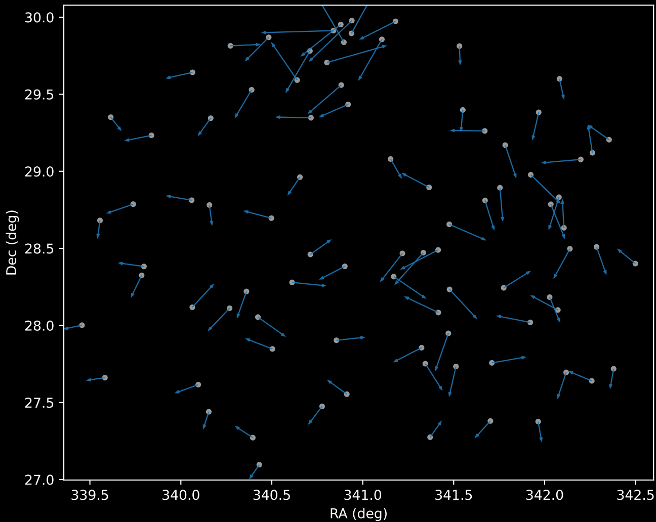
APOGEE DR17 Cluster 0 Proper Motion Vectors (n=87)
