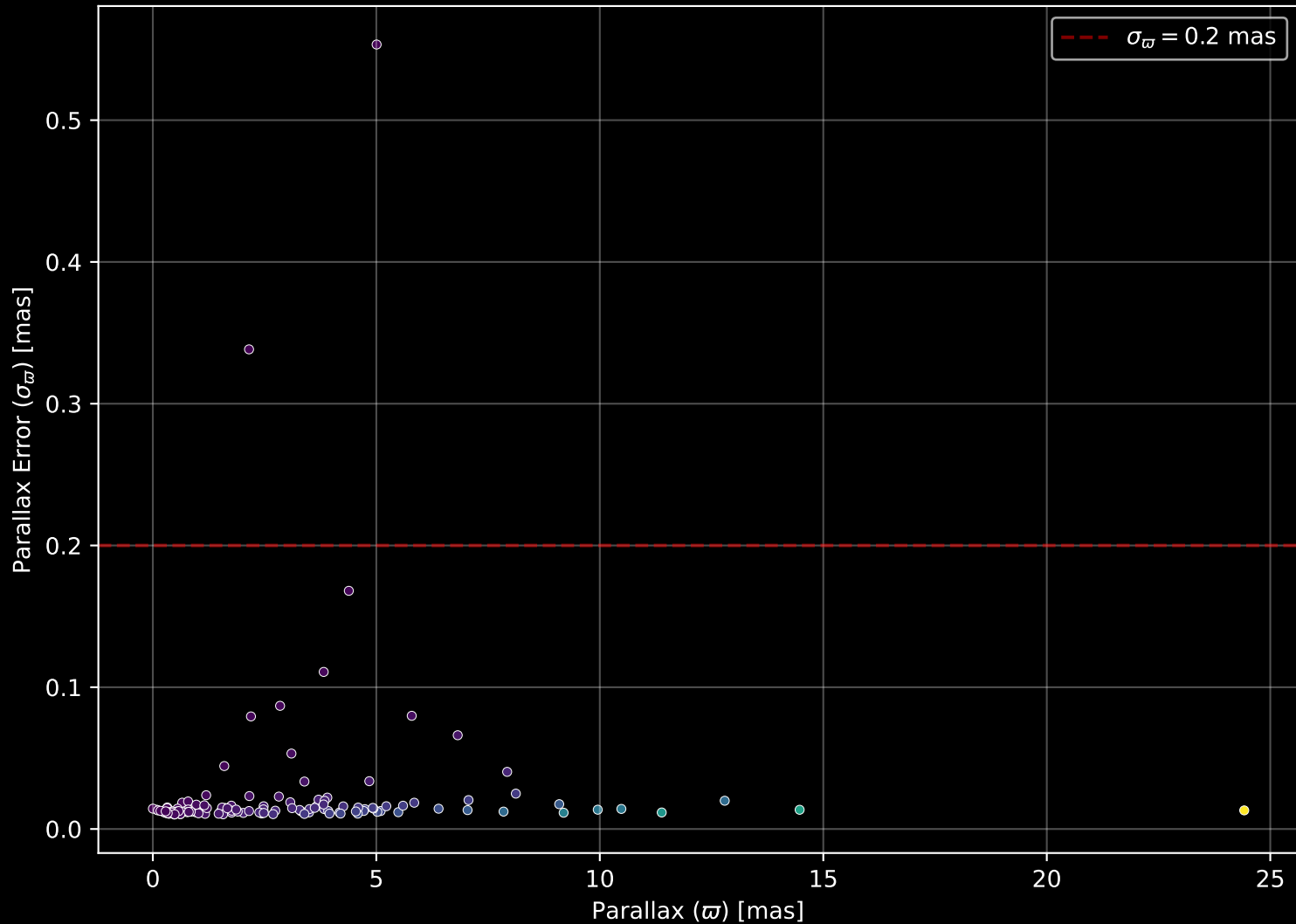
APOGEE DR17 Field: [046+48_MGA] Parallax Quality (n= 129)
