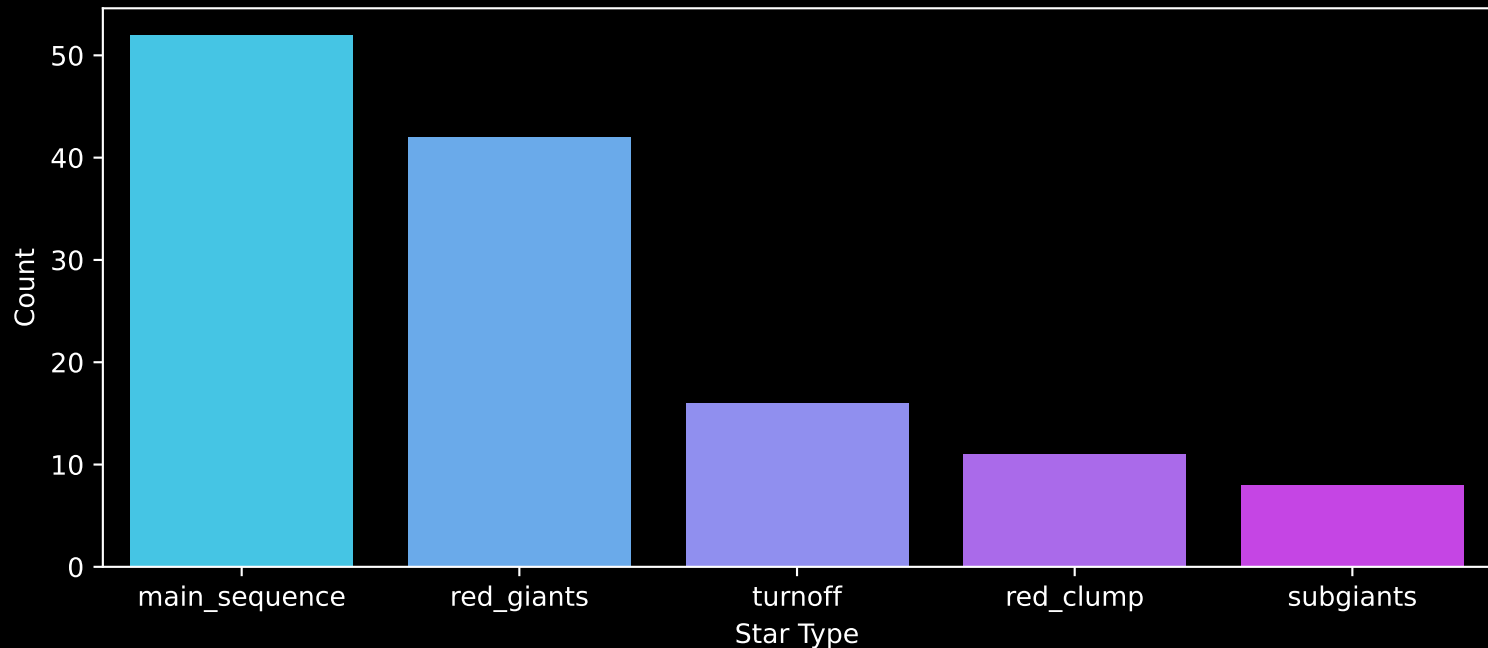
APOGEE DR17 Field: [046+48_MGA] Count plot of Star Type
