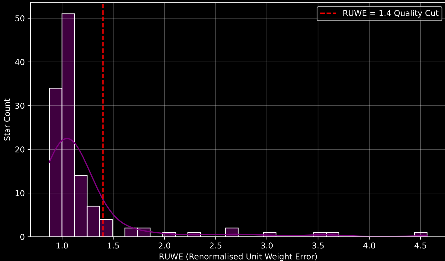
GAPOGEE DR17 Field [046+48_MGA] RUWE Distribution (n= 122)
