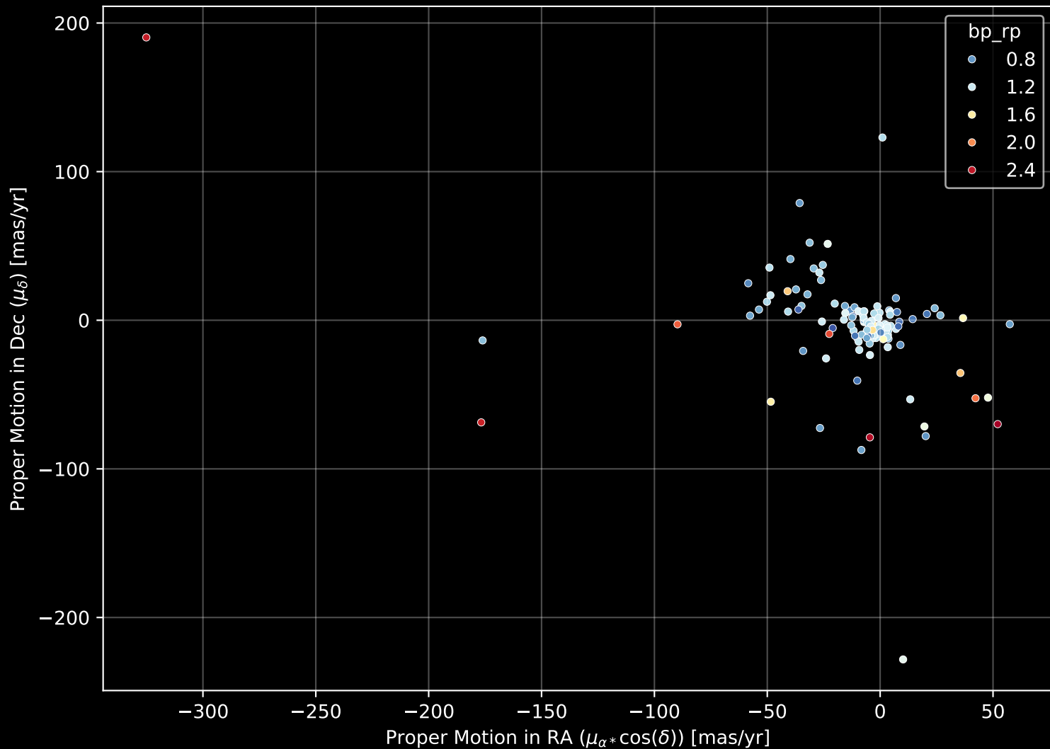
APOGEE DR17 Field: [046+48_MGA] Proper Motion Diagram (n= 129)
