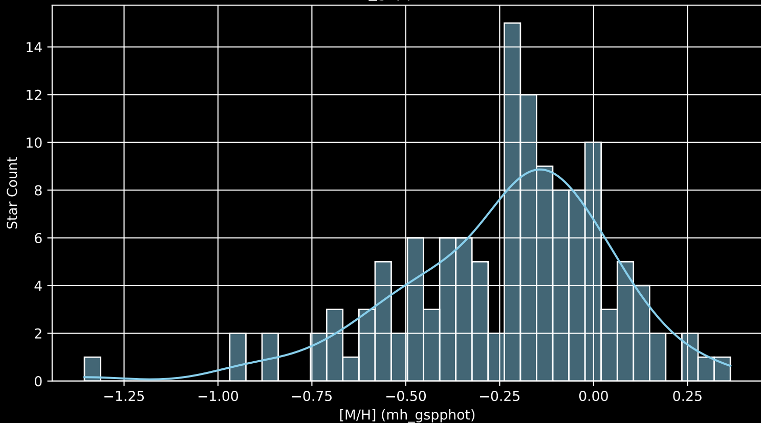
APOGEE DR17 Field: [046+48_MGA [M/H] (mh_gspphot) (n= 129)
